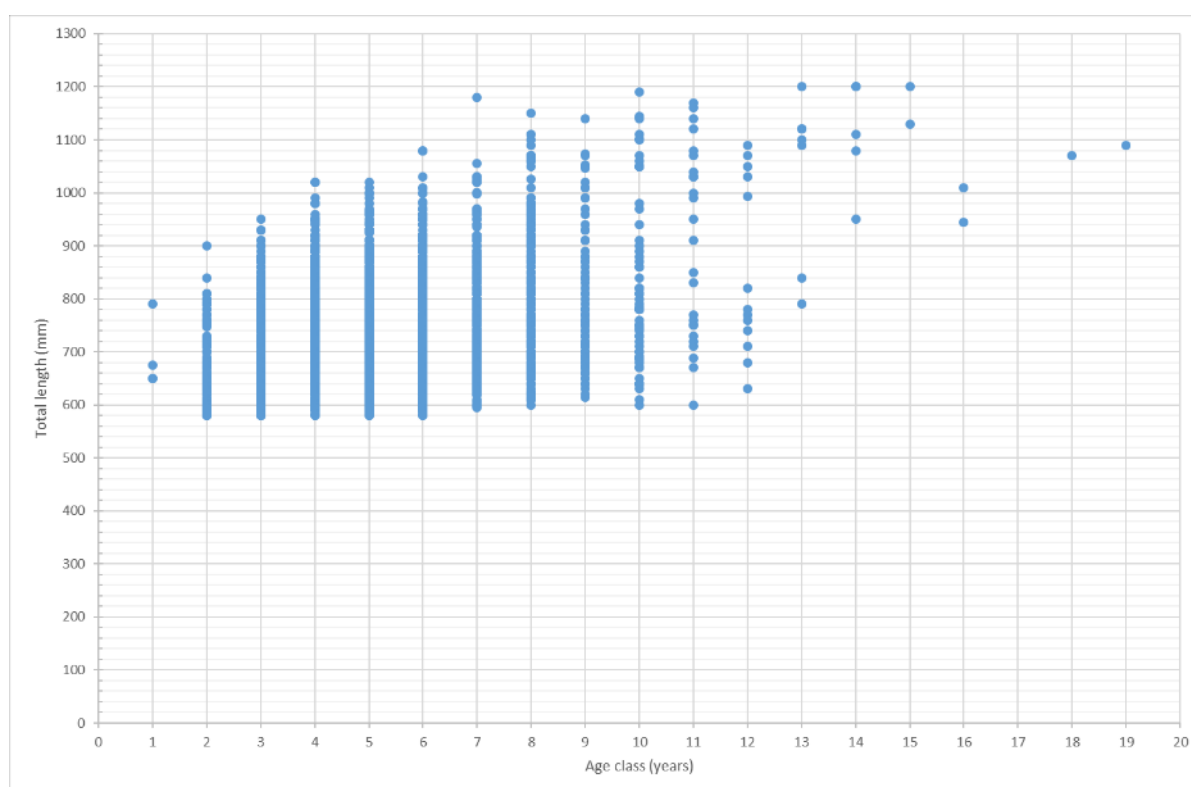
Figure 6-2. Observed length-at-age for legal size barramundi sampled by Department of Agriculture and Fisheries (Queensland) from the mid-region stock between 2000 and 2018 ( n=4,140 ). Figure reproduced from Robins et al. (2021).
