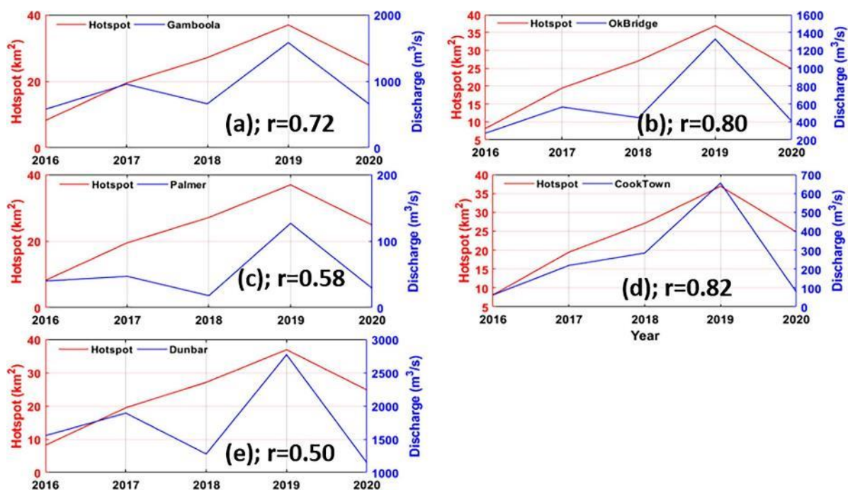
Figure 4-3. Floodplain aquatic plant biomass extent (2016–2020) over the downstream Mitchell catchment, shown as ‘hotspot’ (km²). The relationship between predicted extents of hotspots and observed discharge is indicated for (a) Gamboola, (b) O.K. Bridge, (c) Palmer, (d) Cooktown Crossing and (e) Dunbar. Figure reproduced from Ndehedehe et al. (2021).
