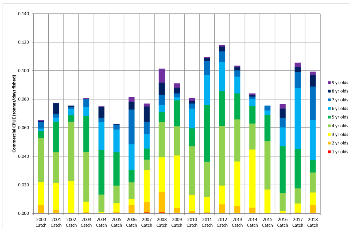
Figure B-2. Estimated age composition of the commercial barramundi catch per year (adjusted for effort) for stock in the Mitchell River influence region. Figure reproduced from Robins et al. (2021).
