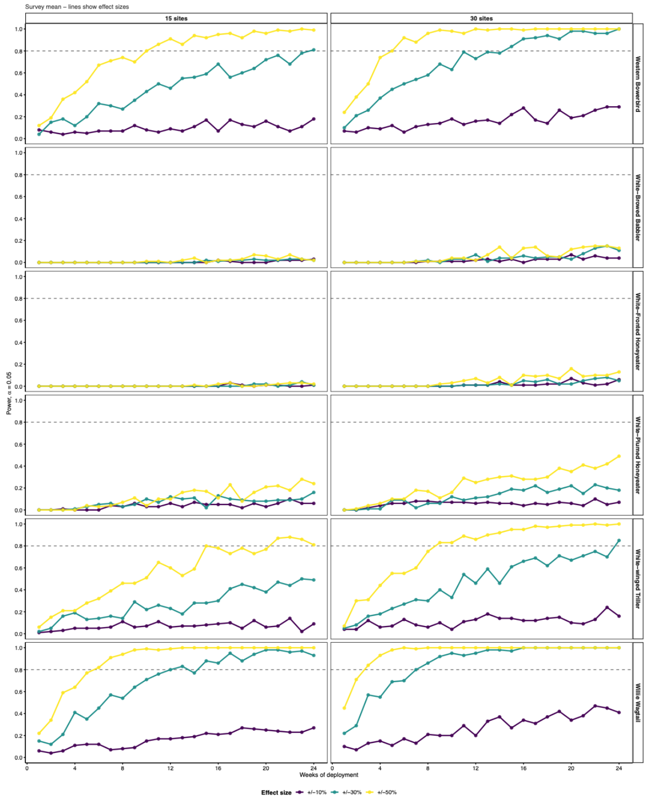
Figure A12. Statistical power to detect a change in encounter rates for all species with sufficient data across varying effect sizes under the current number of survey sites (30) and a halving of survey sites (15). Each row represents a species, with colour indicating the simulated effects size number of survey weeks (x-axis). The y-axis shows the statistical power for a given site number (column) and survey effort.
