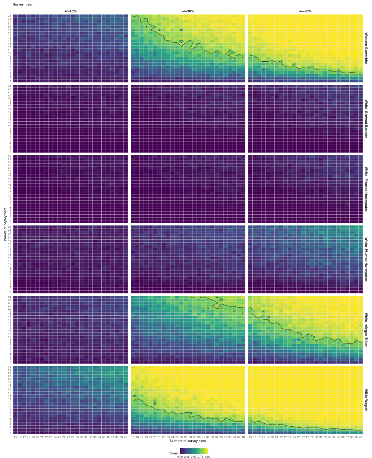
Figure A10. Statistical power to detect a change in encounter for each species across varying effect sizes and survey effort. Each row represents a species, with colour indicating the proportion of simulations (0–1) achieving statistical significance ( \alpha = 0.05 ) for a given combination of effect size (columns) and number of survey sites (x-axis). The y-axis shows the number of survey weeks, and contour lines denote power thresholds (0.8 shown in black).
