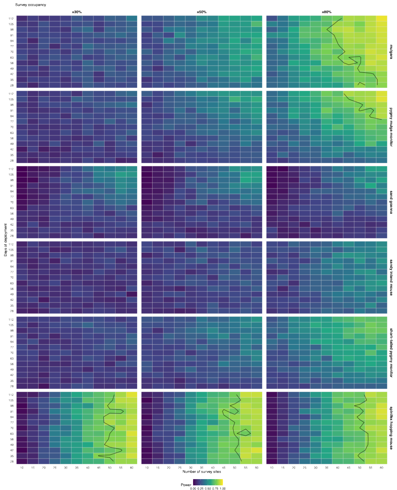
Figure A9. Statistical power to detect a change in site level occupancy for each species across varying effect sizes and survey effort. Each row represents a species, with colour indicating the proportion of simulations (0–1) achieving statistical significance ( \alpha = 0.05 ) for a given combination of effect size (columns) and number of survey sites (x-axis). The y-axis shows the number of survey sessions, and contour lines denote power thresholds (0.8 shown in black). Red markers highlight conditions achieving \geq 80\% power.
